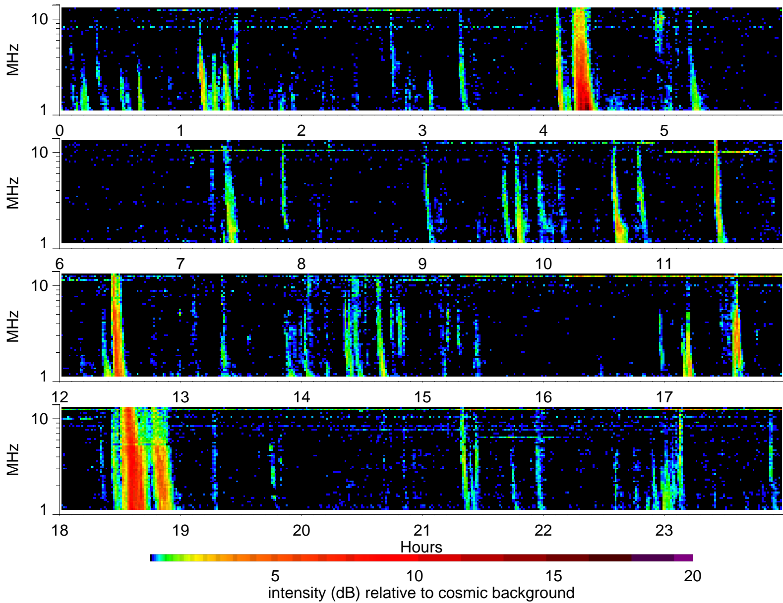
Wind Waves RAD2 receiver: 2001/9/2
