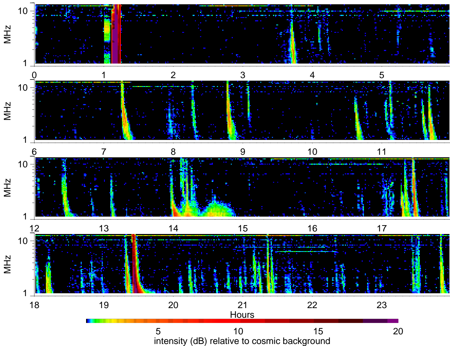
Wind Waves RAD2 receiver: 2001/9/1
