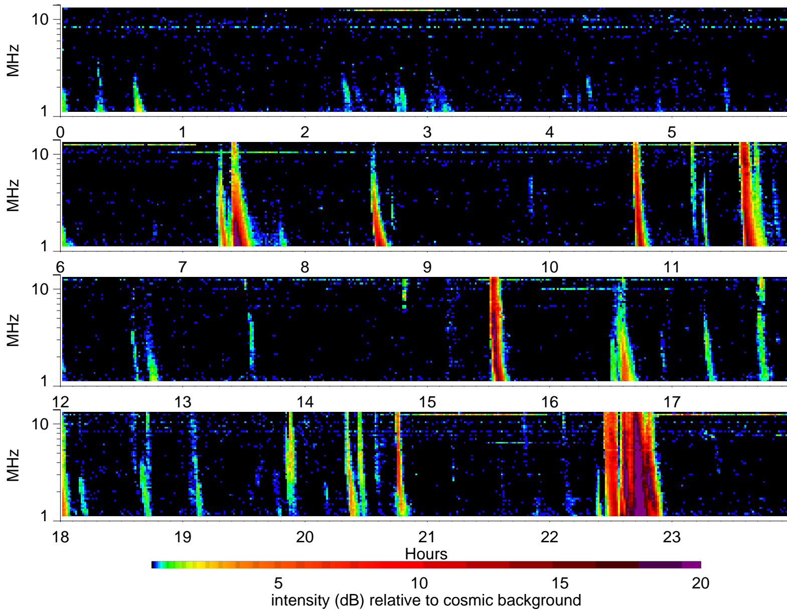
Wind Waves RAD2 receiver: 2001/8/31
