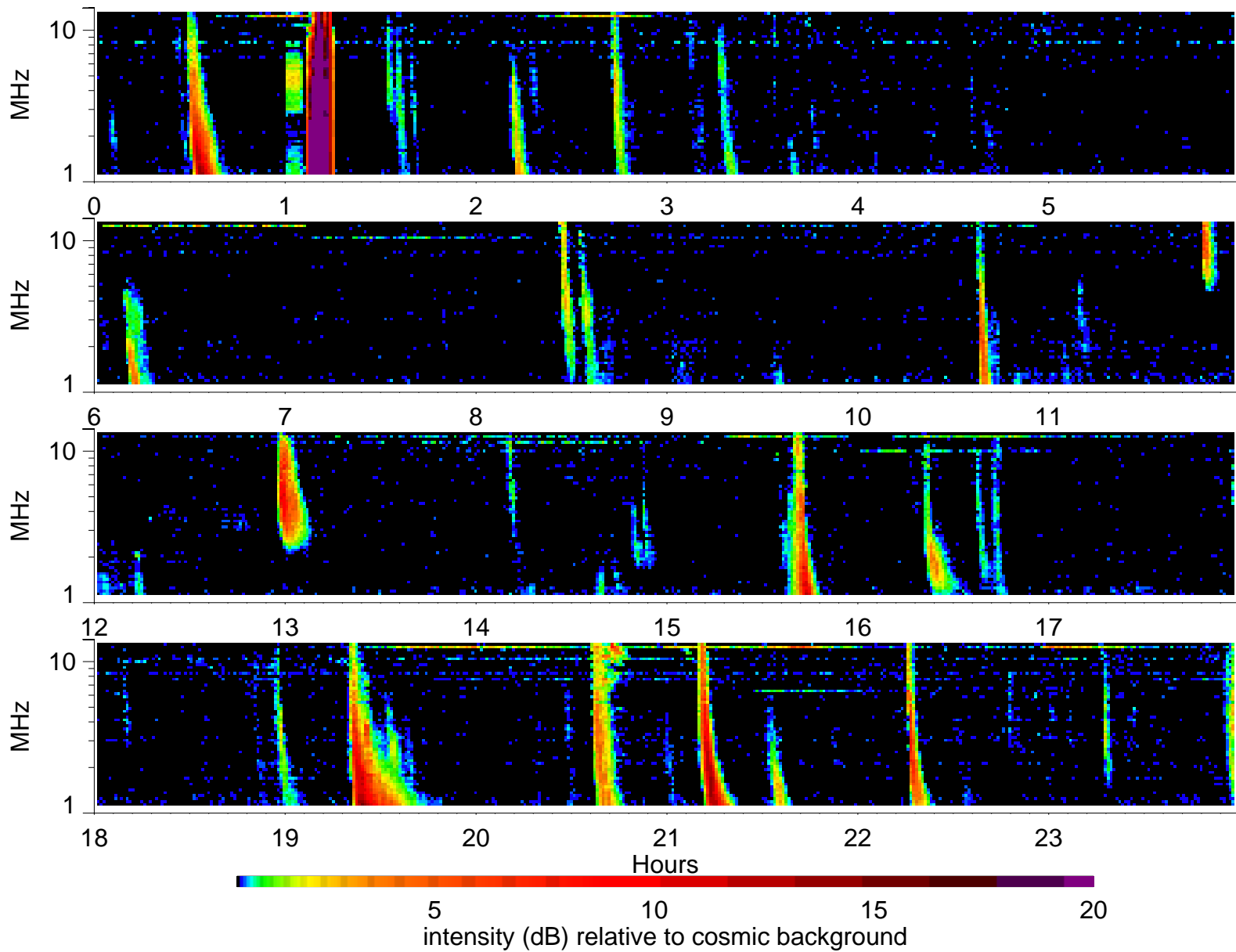
Wind Waves RAD2 receiver: 2001/8/30
