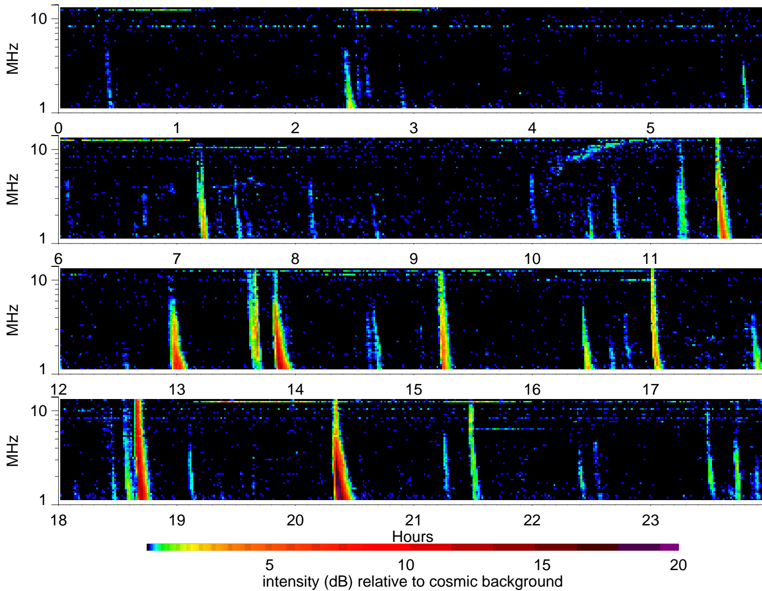
Wind Waves RAD2 receiver: 2001/8/29
