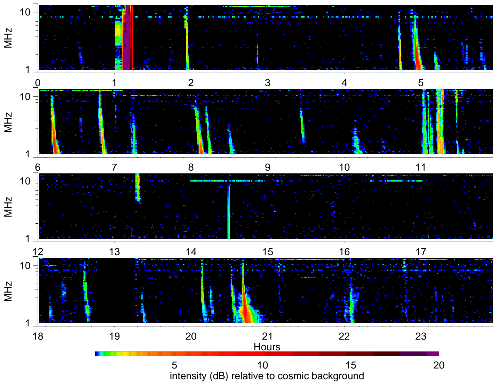
Wind Waves RAD2 receiver: 2001/8/24
