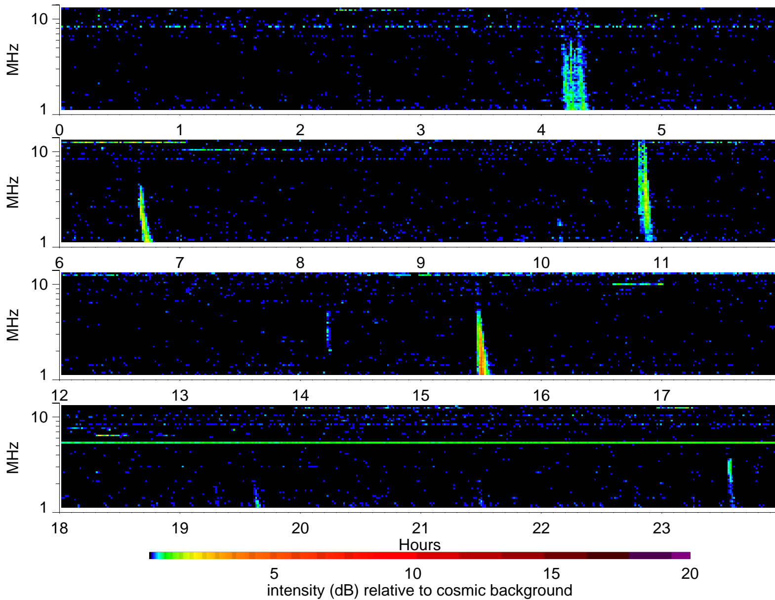
Wind Waves RAD2 receiver: 2001/8/19
