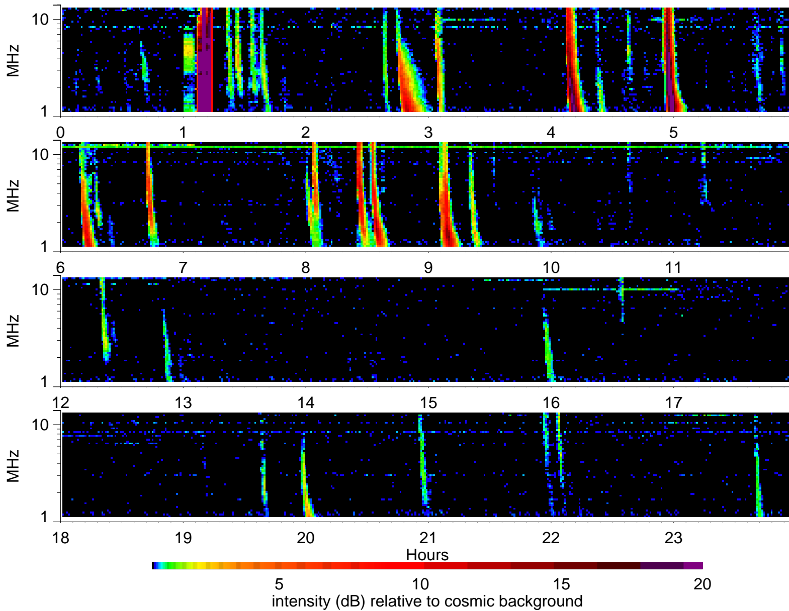
Wind Waves RAD2 receiver: 2001/8/10
