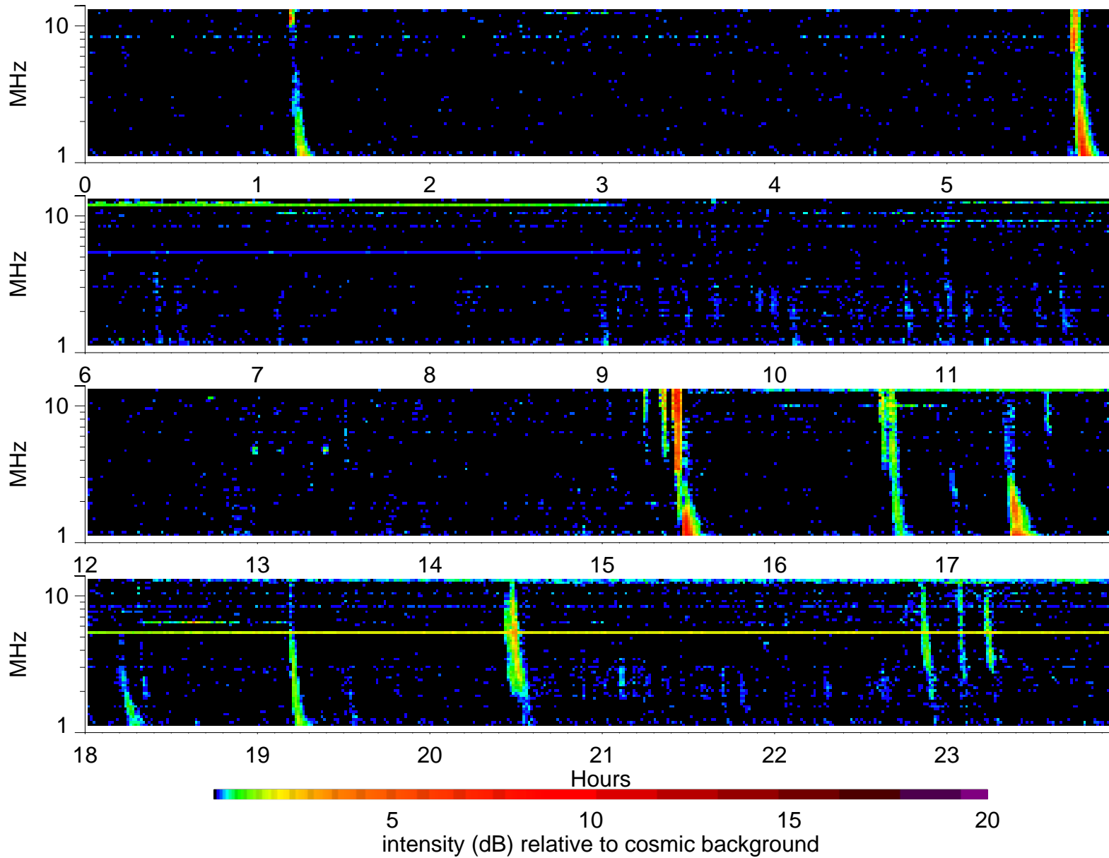
Wind Waves RAD2 receiver: 2001/8/9
