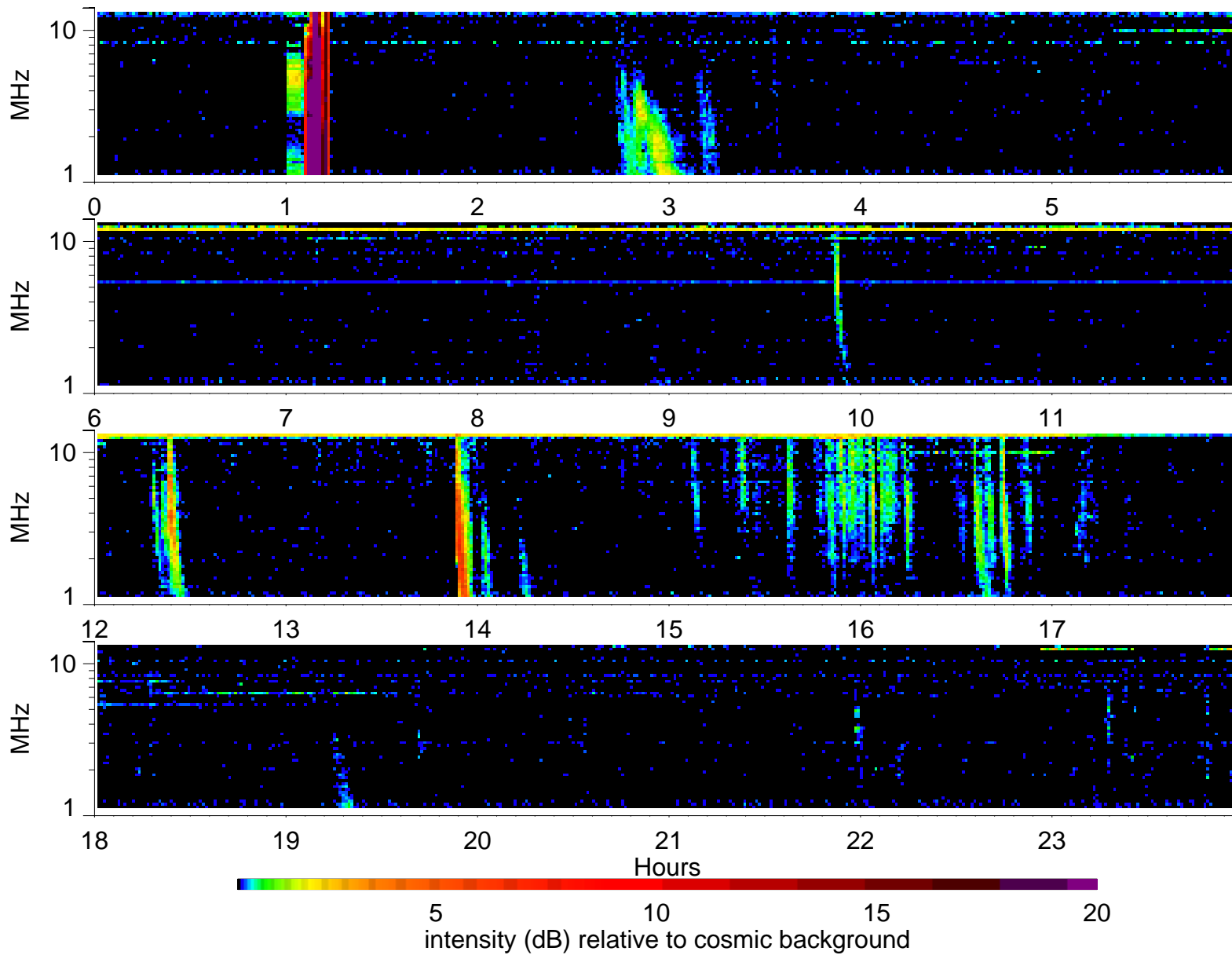
Wind Waves RAD2 receiver: 2001/8/6
