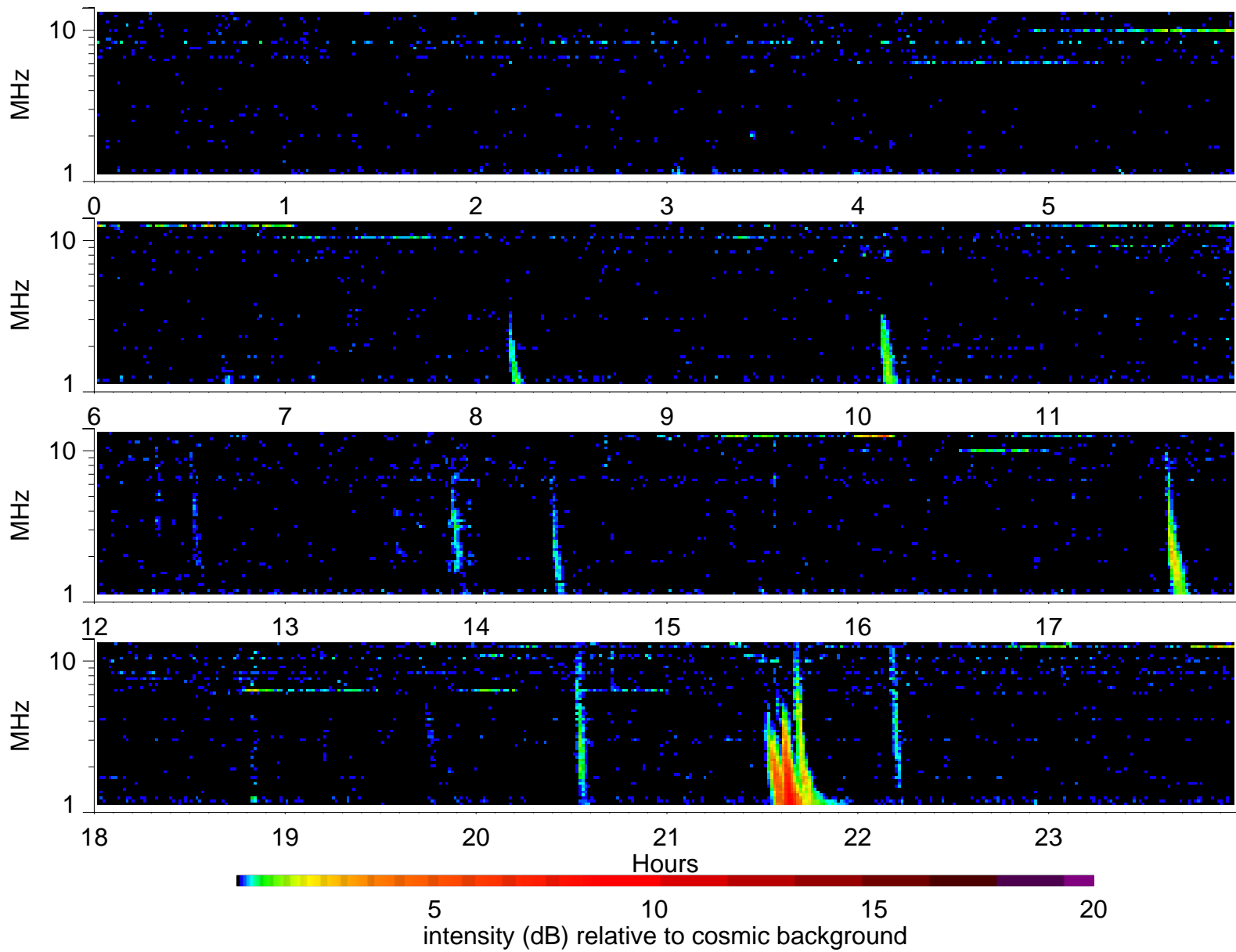
Wind Waves RAD2 receiver: 2001/8/5
