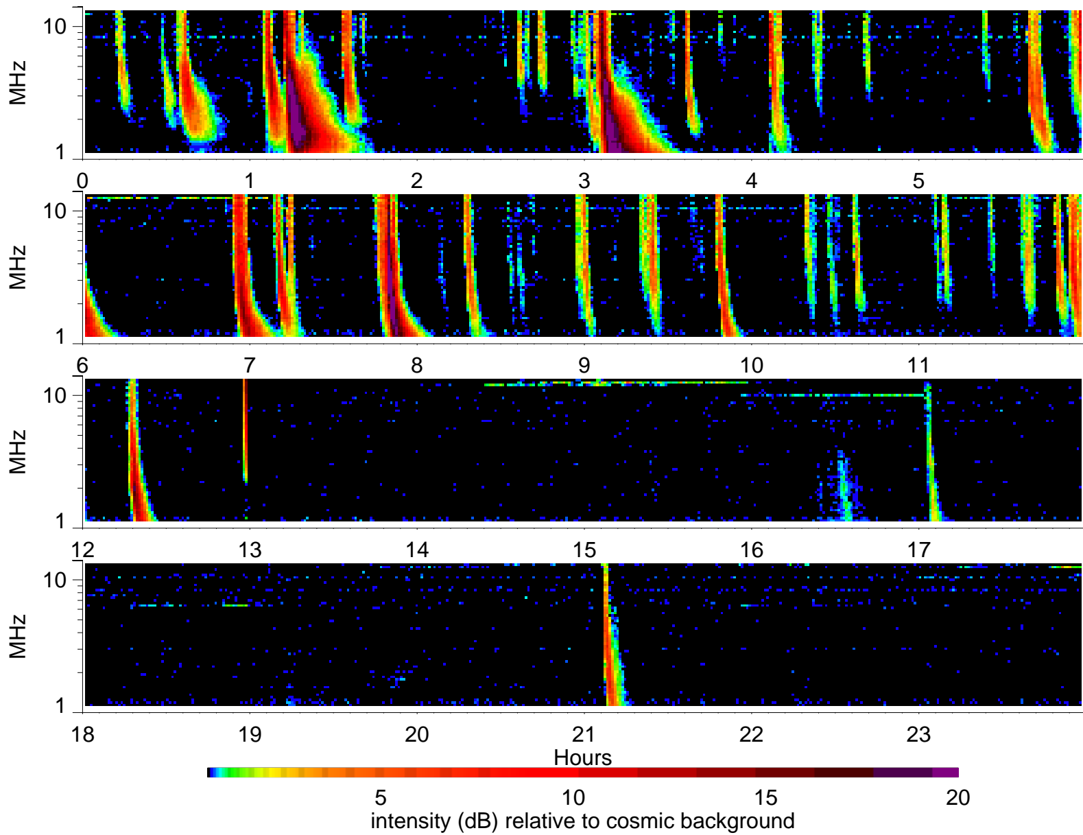
Wind Waves RAD2 receiver: 2001/8/3
