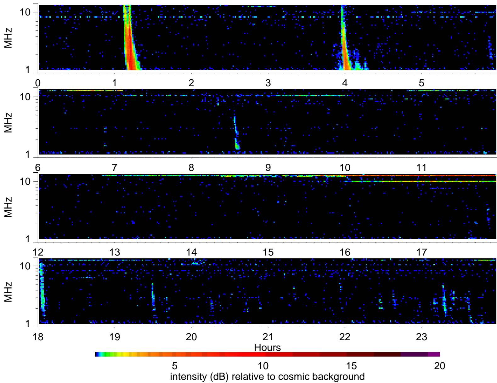
Wind Waves RAD2 receiver: 2001/8/1
