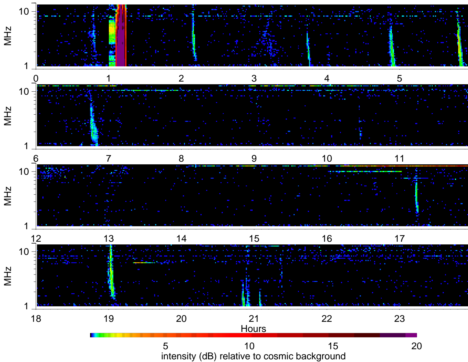
Wind Waves RAD2 receiver: 2001/7/27
