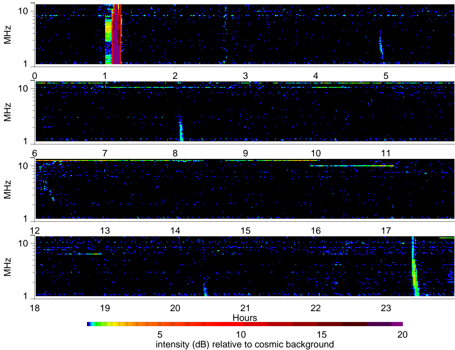
Wind Waves RAD2 receiver: 2001/7/21
