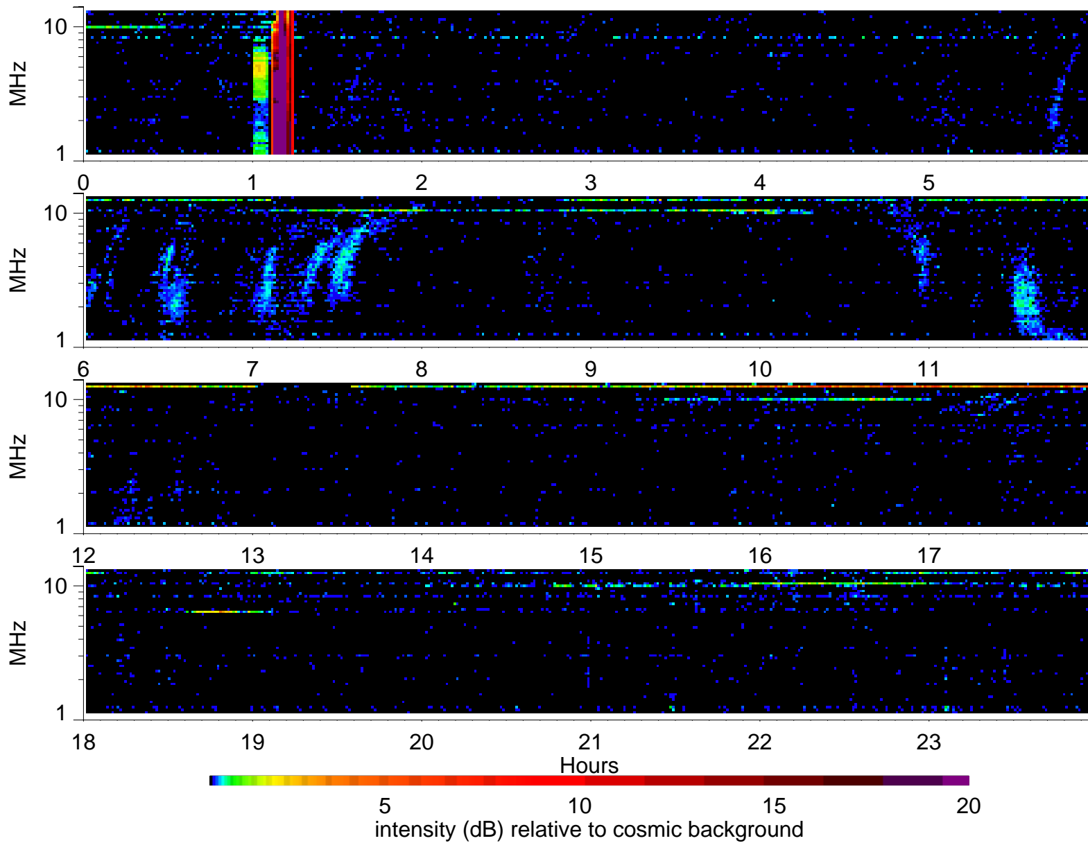
Wind Waves RAD2 receiver: 2001/7/17
