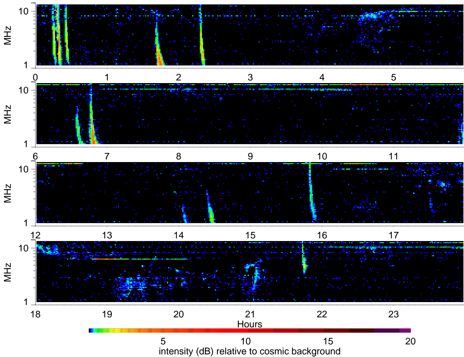
Wind Waves RAD2 receiver: 2001/7/16
