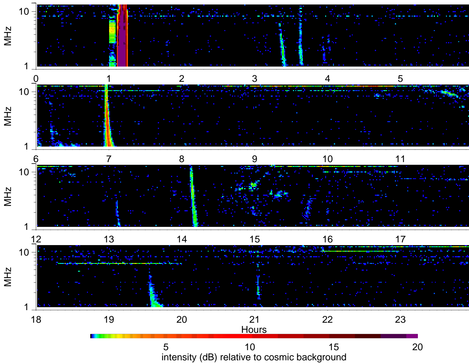
Wind Waves RAD2 receiver: 2001/7/15
