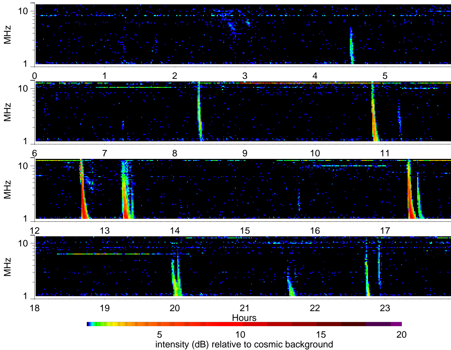
Wind Waves RAD2 receiver: 2001/7/14
