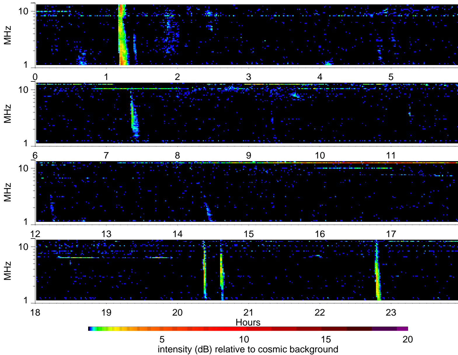
Wind Waves RAD2 receiver: 2001/7/12
