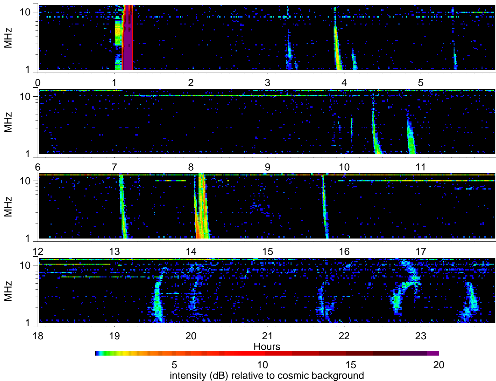
Wind Waves RAD2 receiver: 2001/7/11
