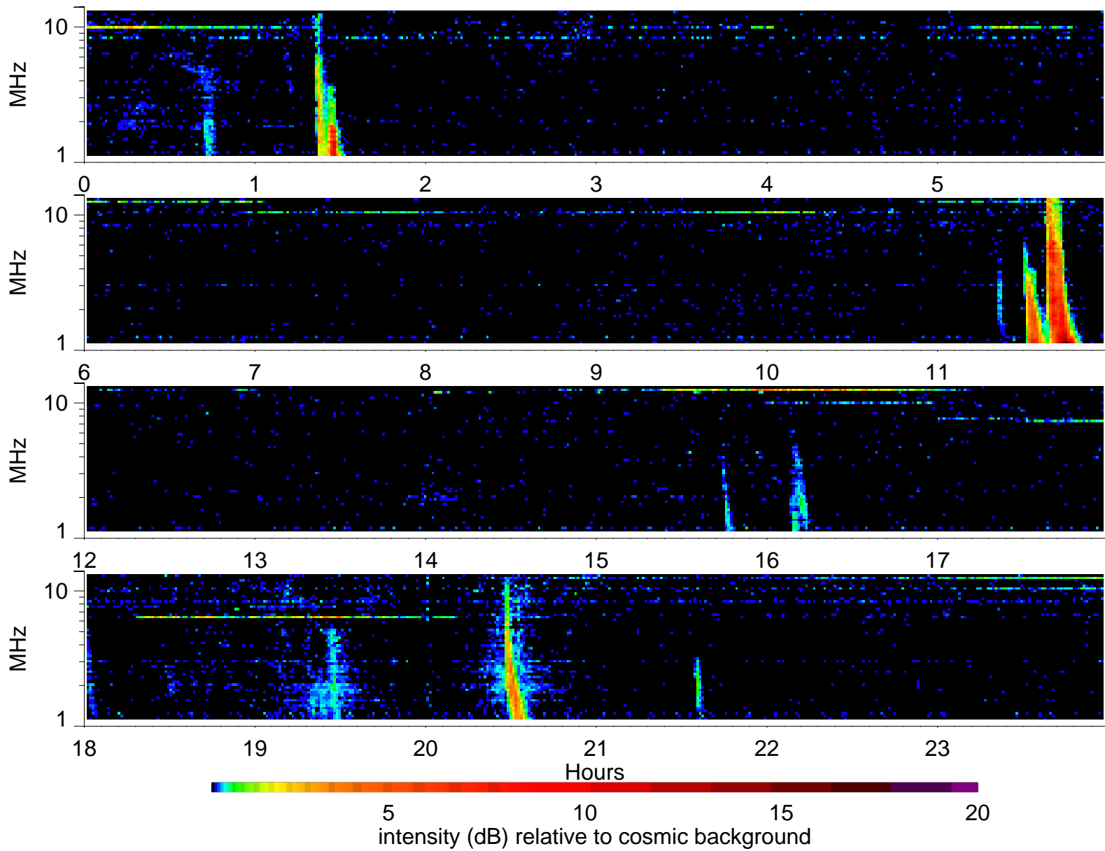
Wind Waves RAD2 receiver: 2001/7/8
