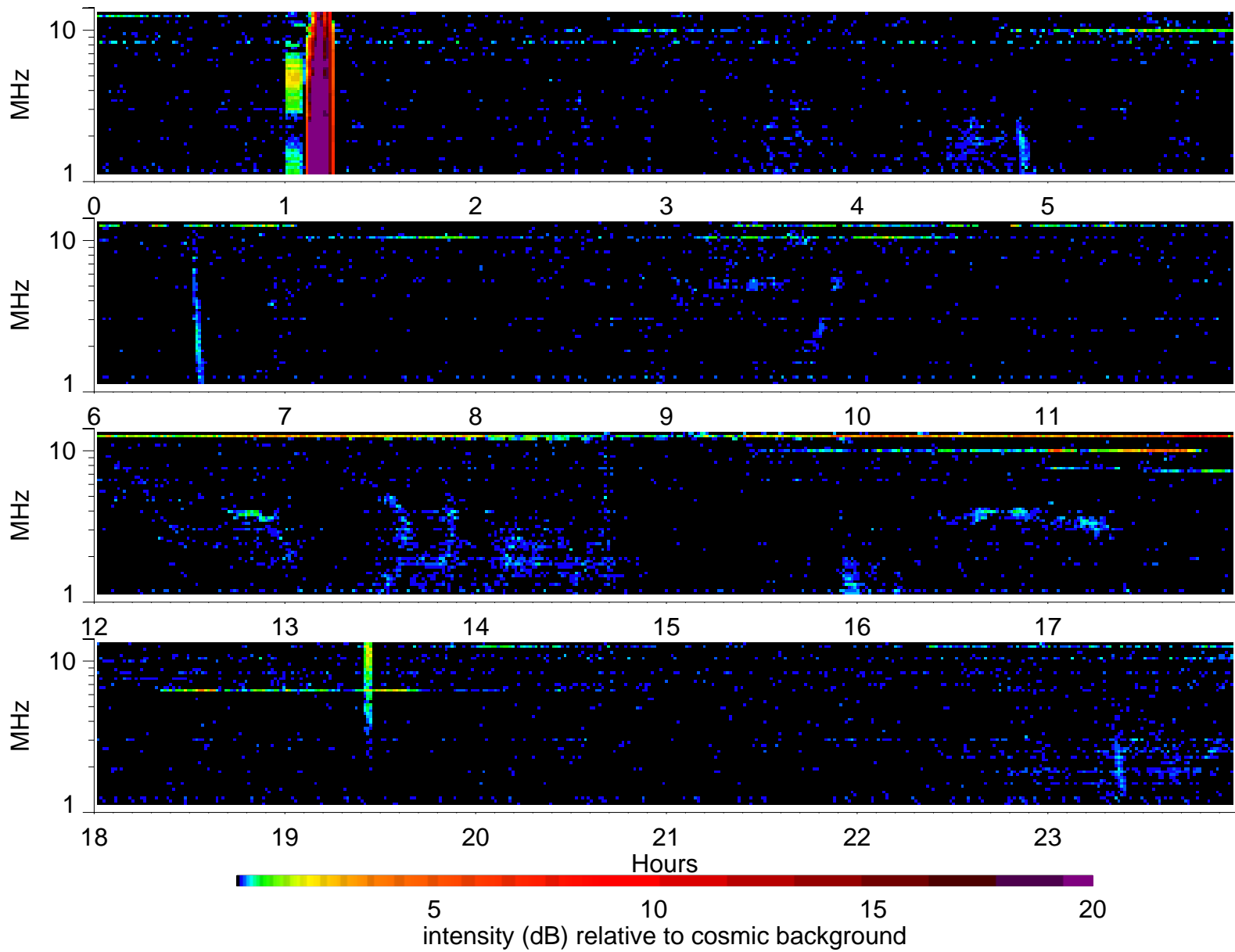
Wind Waves RAD2 receiver: 2001/7/7
