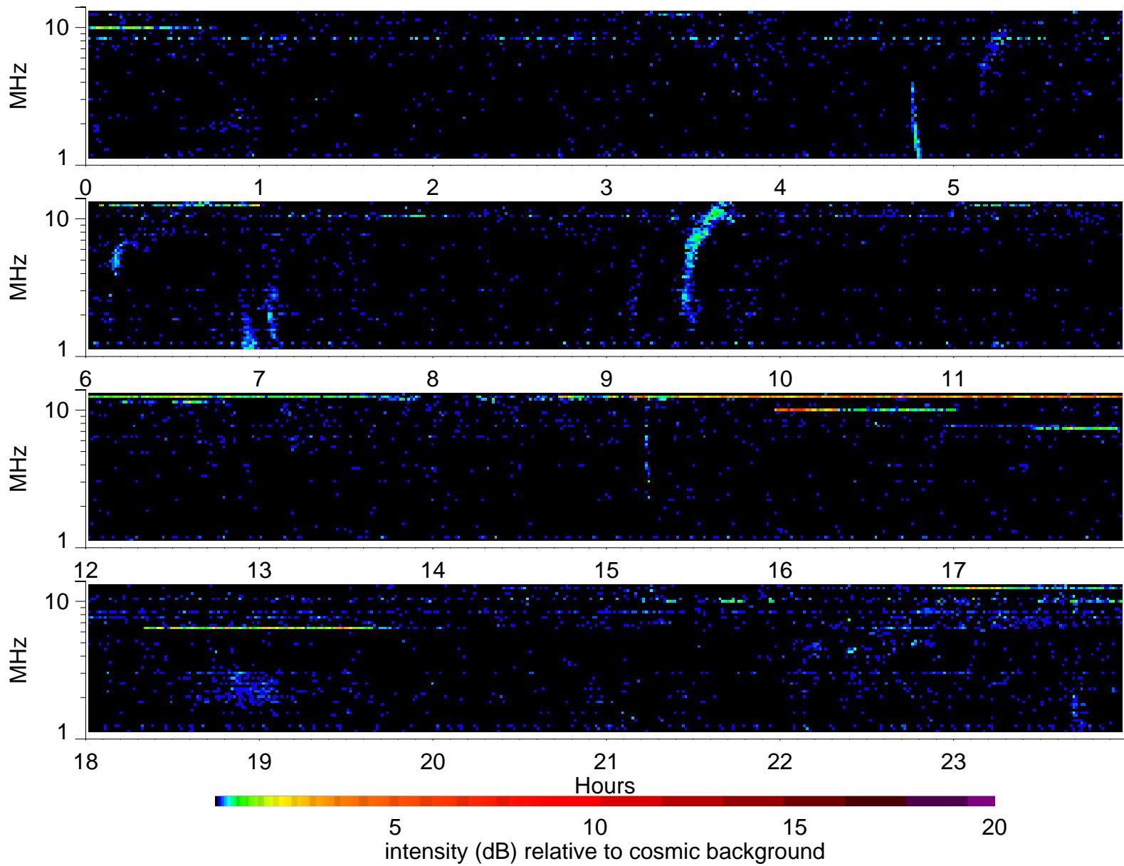
Wind Waves RAD2 receiver: 2001/7/6
