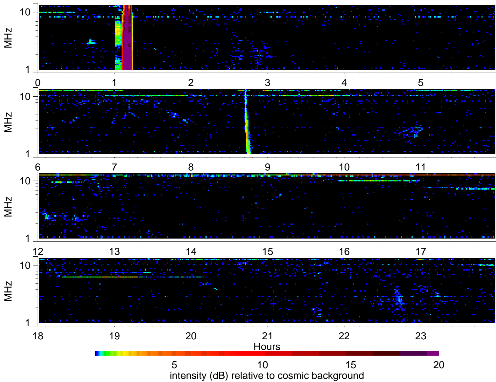
Wind Waves RAD2 receiver: 2001/7/5
