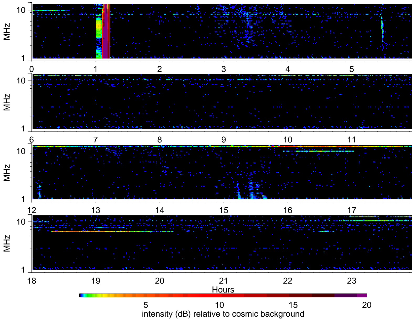
Wind Waves RAD2 receiver: 2001/6/29
