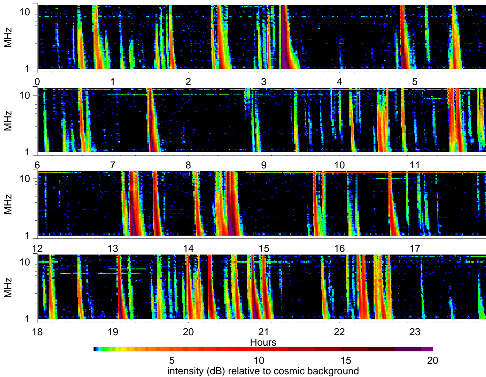
Wind Waves RAD2 receiver: 2001/6/24
