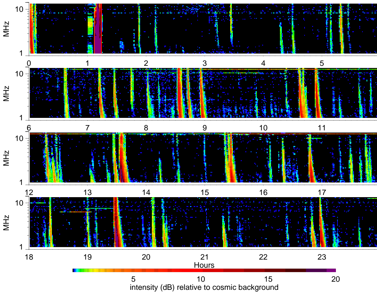
Wind Waves RAD2 receiver: 2001/6/23
