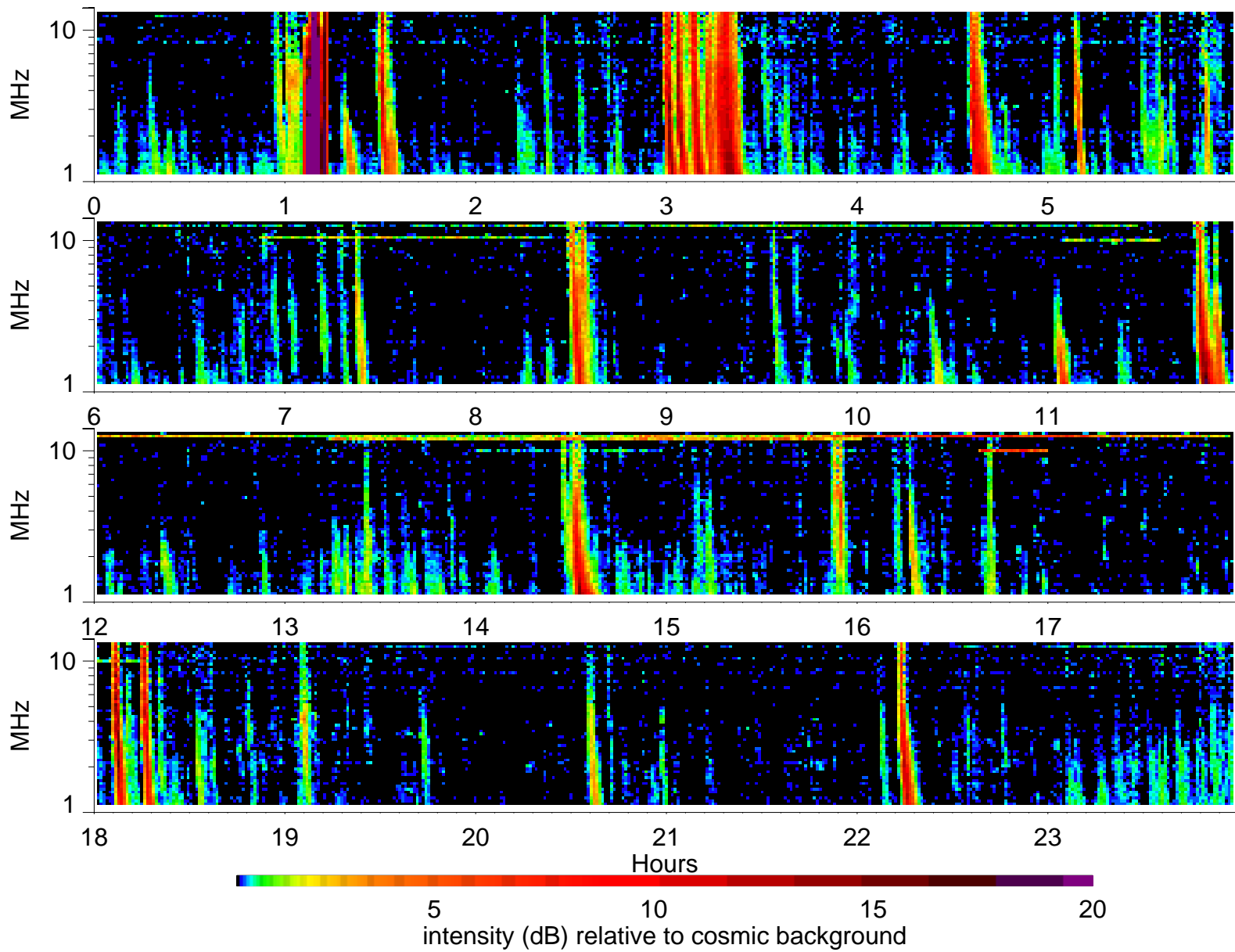
Wind Waves RAD2 receiver: 2001/6/21
