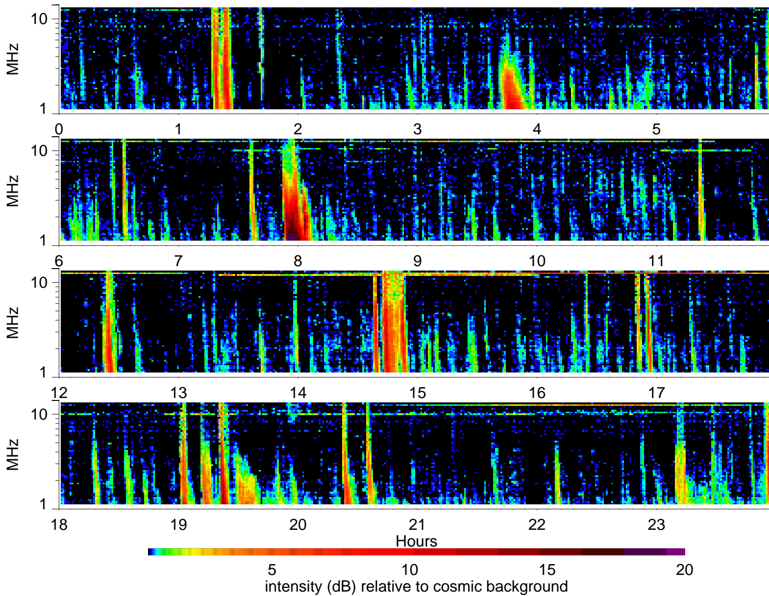
Wind Waves RAD2 receiver: 2001/6/20
