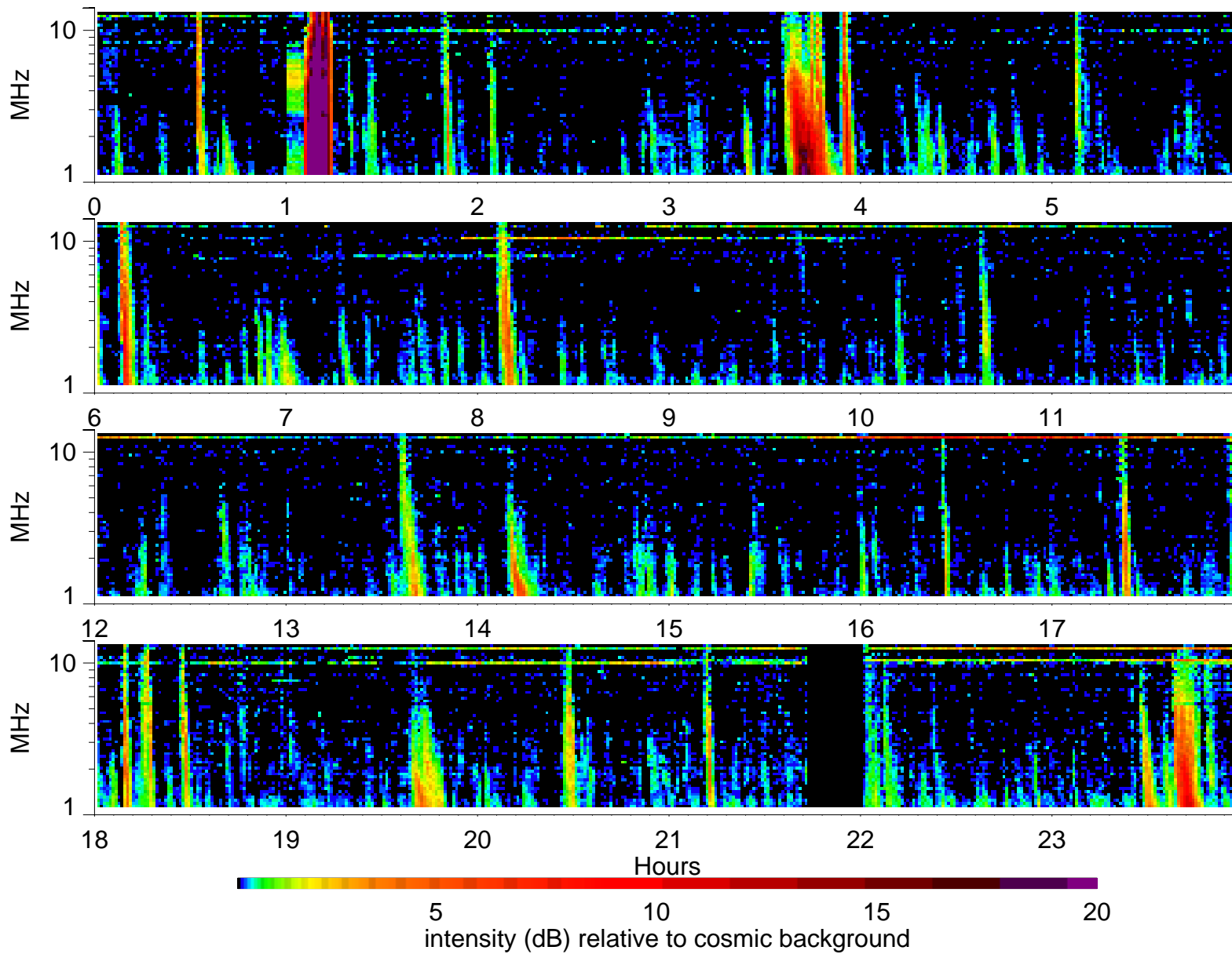
Wind Waves RAD2 receiver: 2001/6/19
