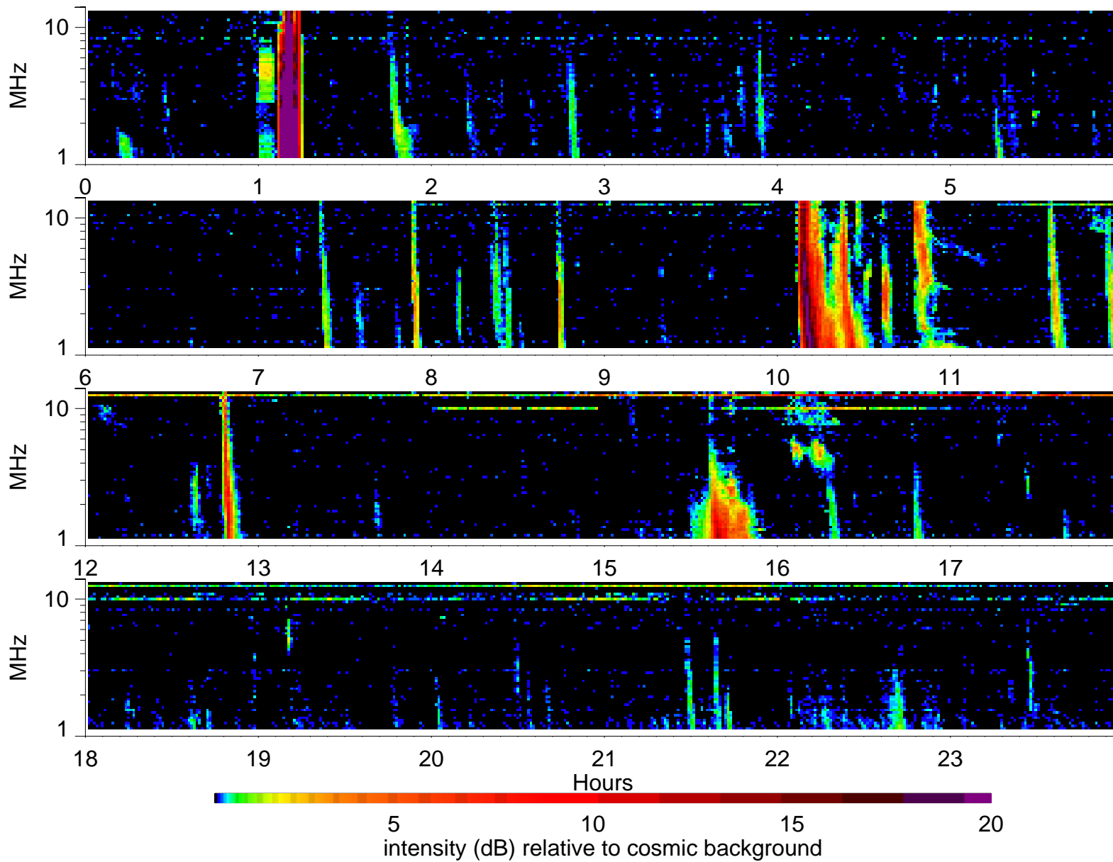
Wind Waves RAD2 receiver: 2001/6/15
