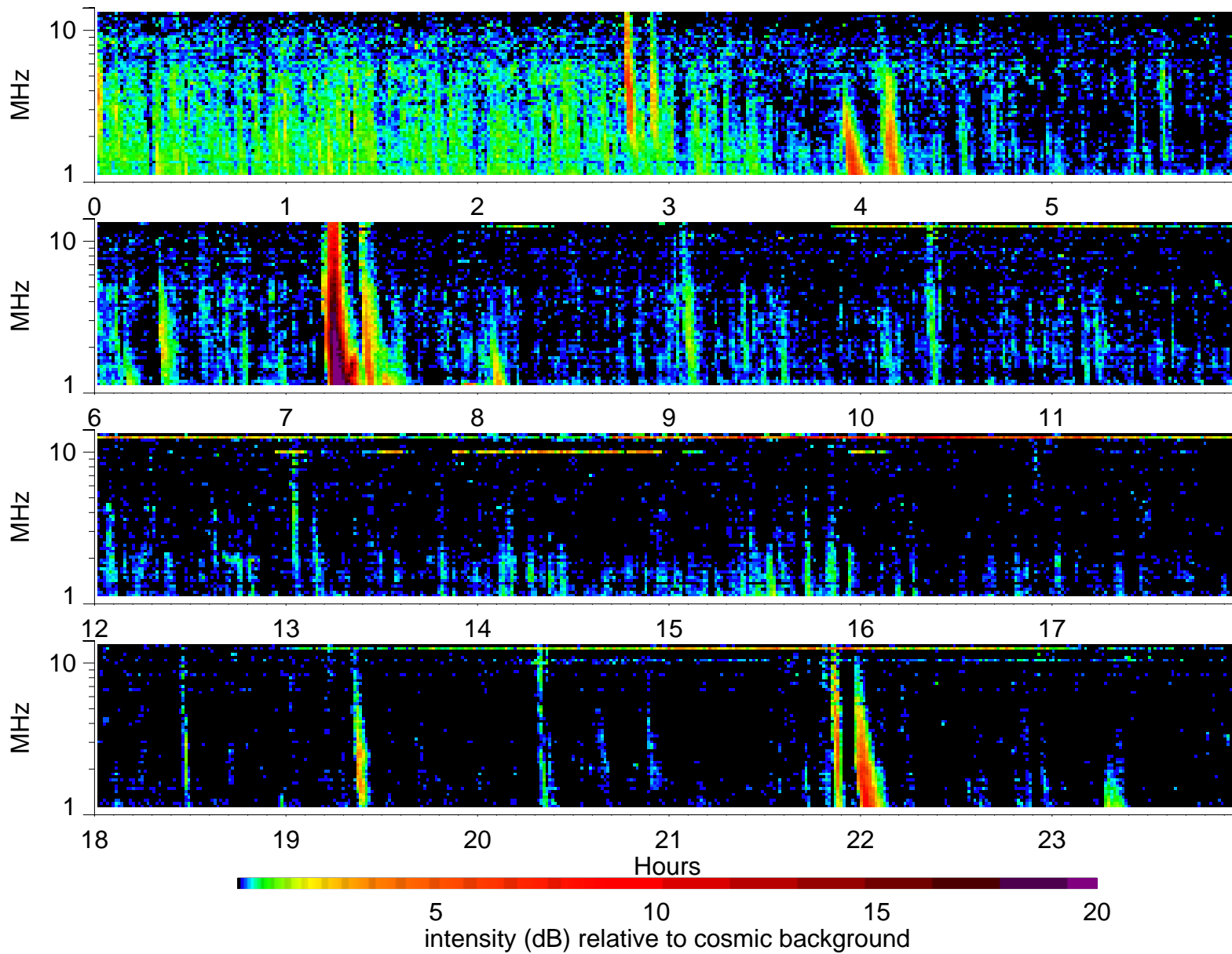
Wind Waves RAD2 receiver: 2001/6/12
