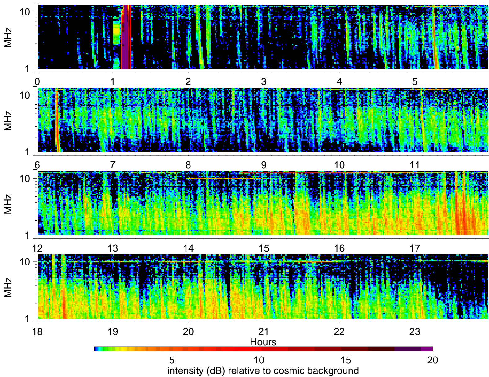
Wind Waves RAD2 receiver: 2001/6/9
