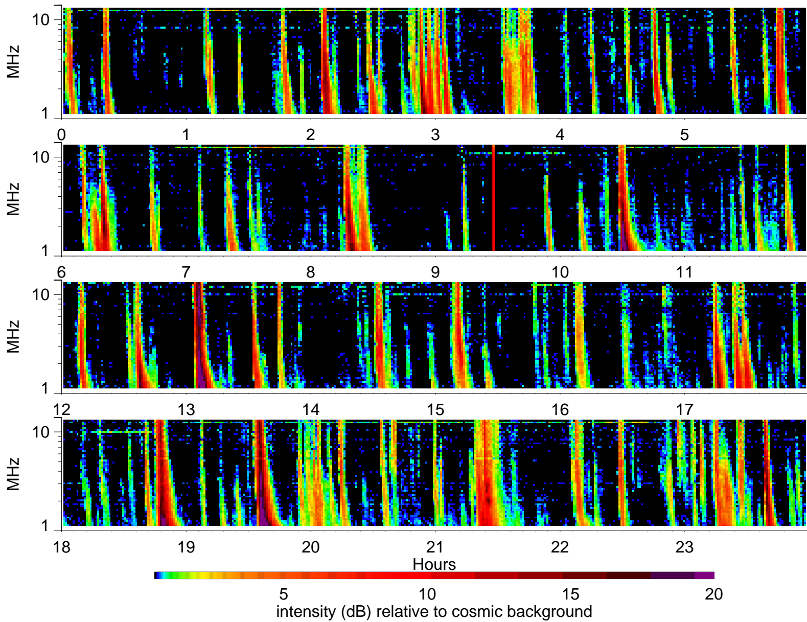
Wind Waves RAD2 receiver: 2001/6/6
