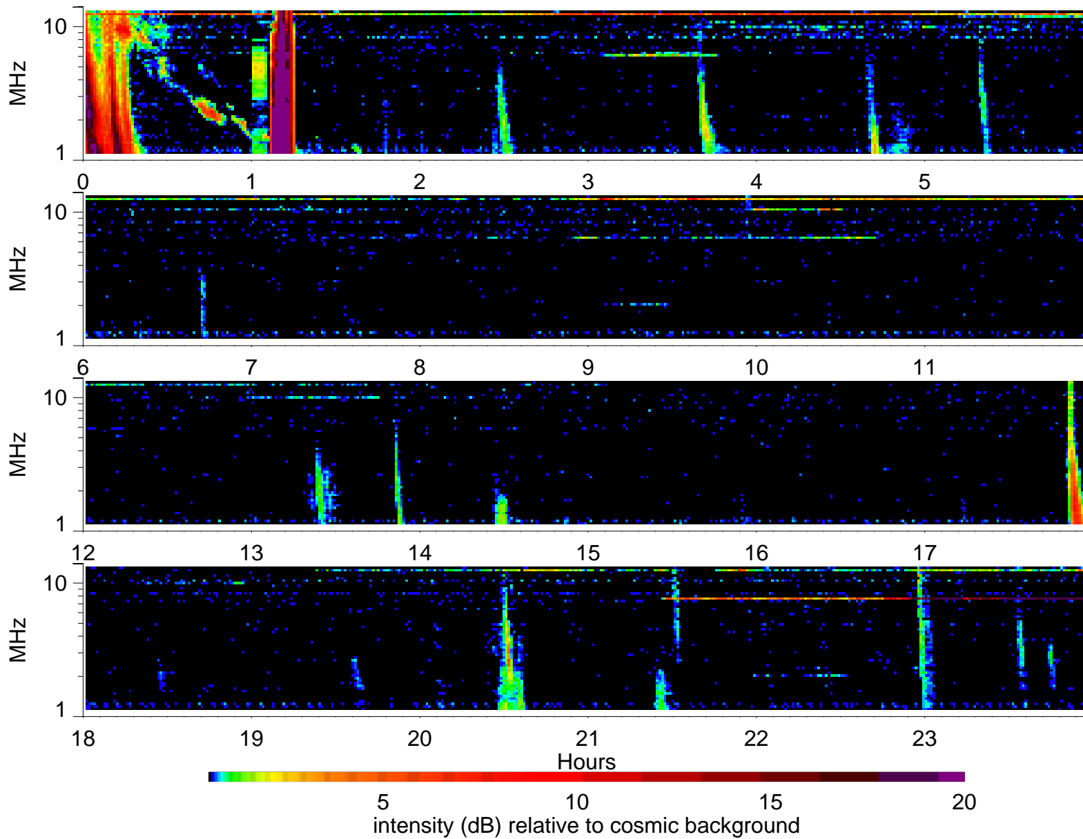
Wind Waves RAD2 receiver: 2001/5/30
