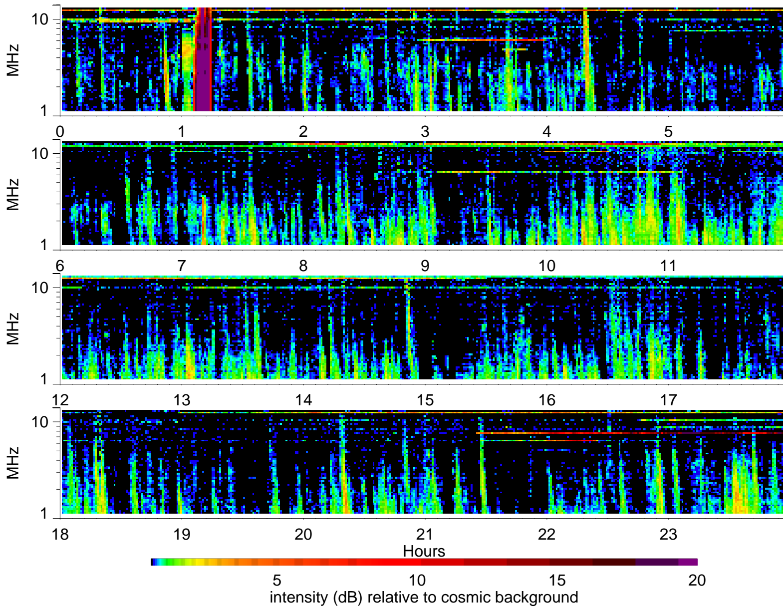
Wind Waves RAD2 receiver: 2001/5/26
