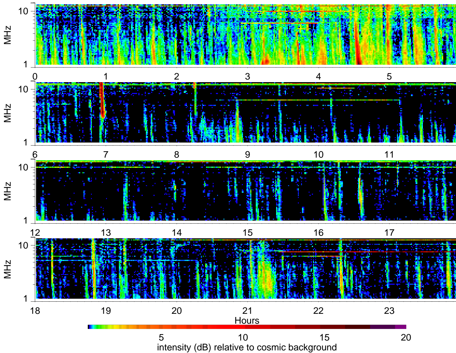
Wind Waves RAD2 receiver: 2001/5/25
