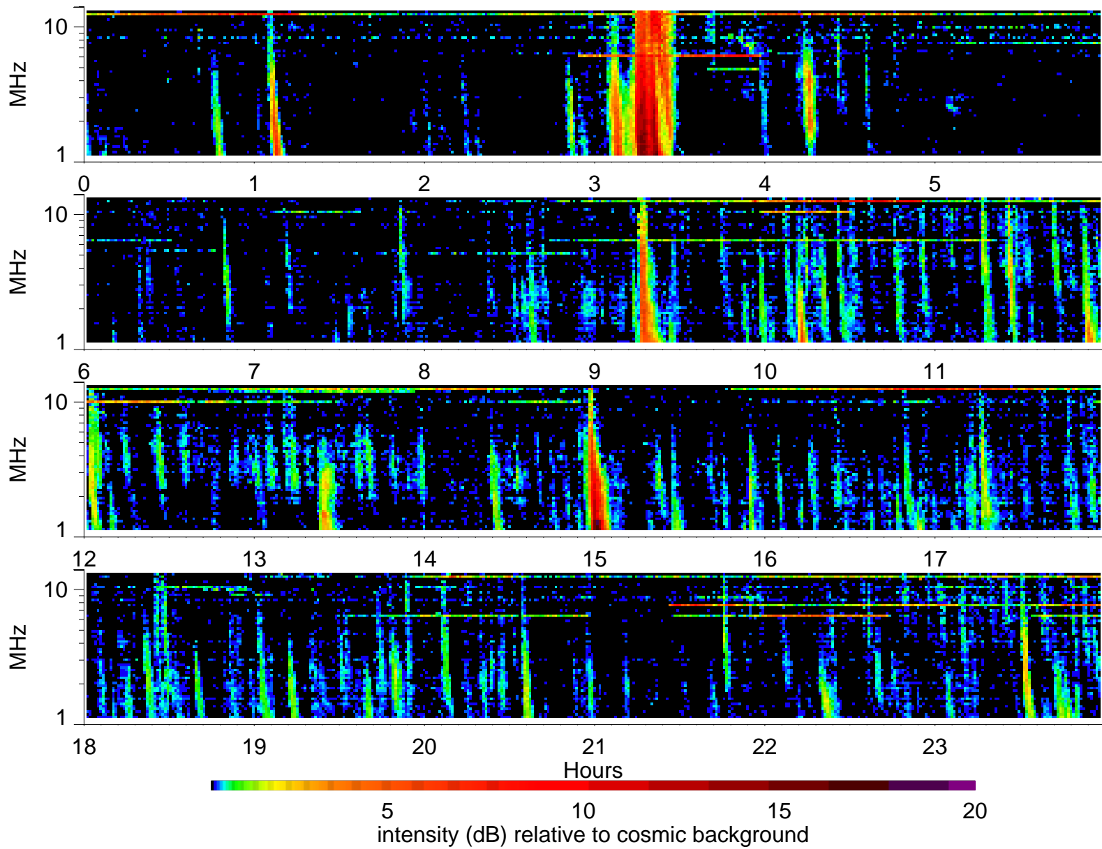
Wind Waves RAD2 receiver: 2001/5/21
