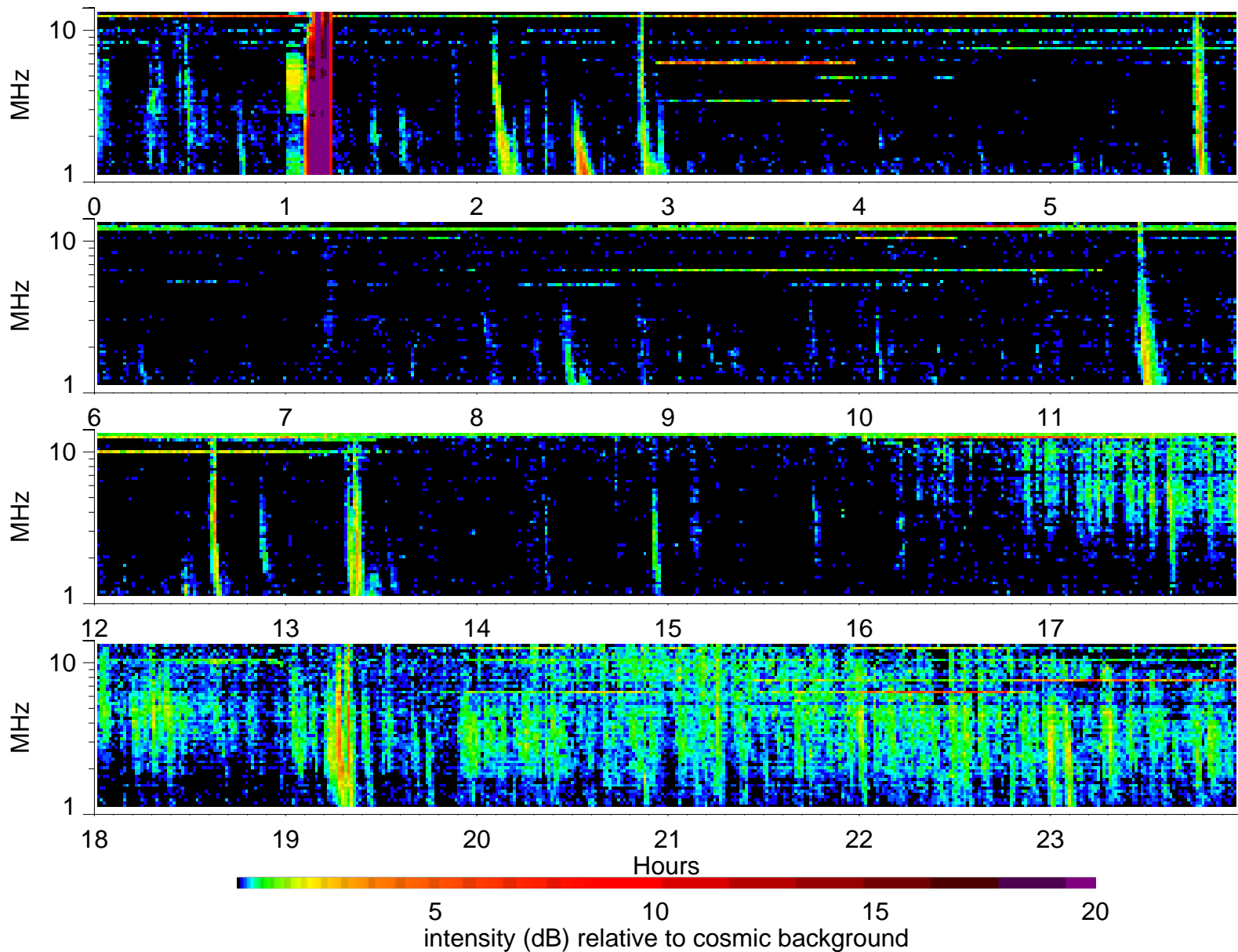
Wind Waves RAD2 receiver: 2001/5/18
