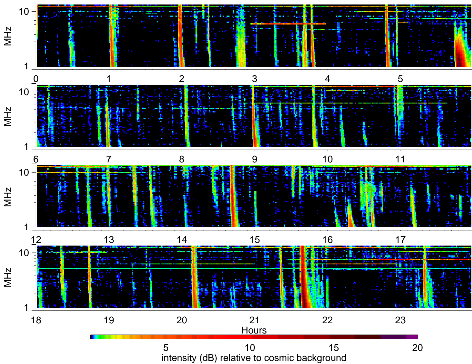
Wind Waves RAD2 receiver: 2001/5/17
