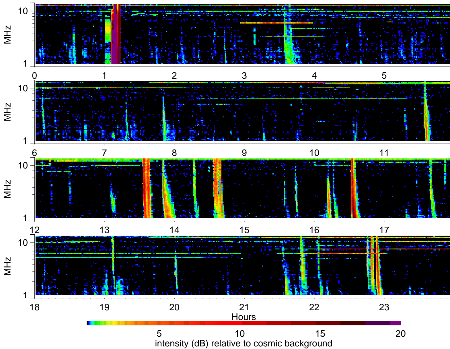
Wind Waves RAD2 receiver: 2001/5/14
