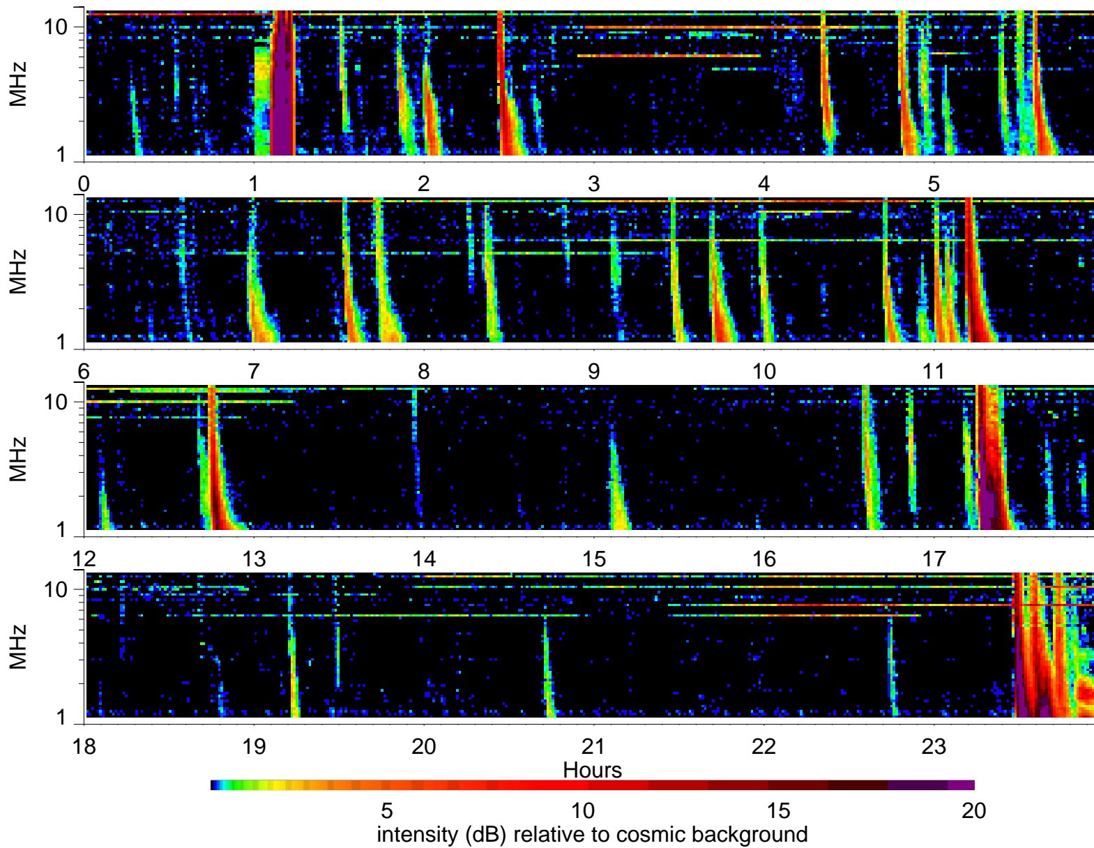
Wind Waves RAD2 receiver: 2001/5/12
