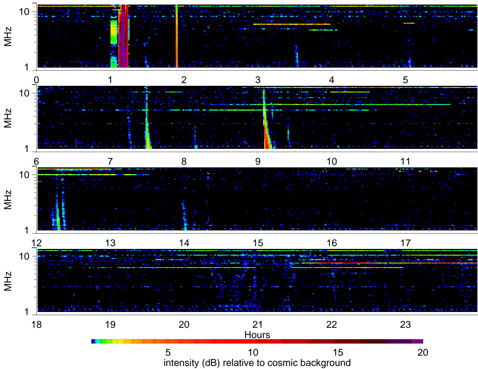
Wind Waves RAD2 receiver: 2001/5/8
