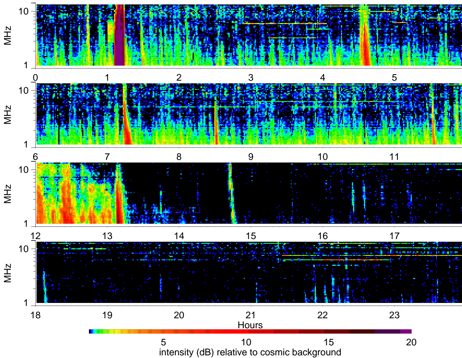
Wind Waves RAD2 receiver: 2001/4/26
