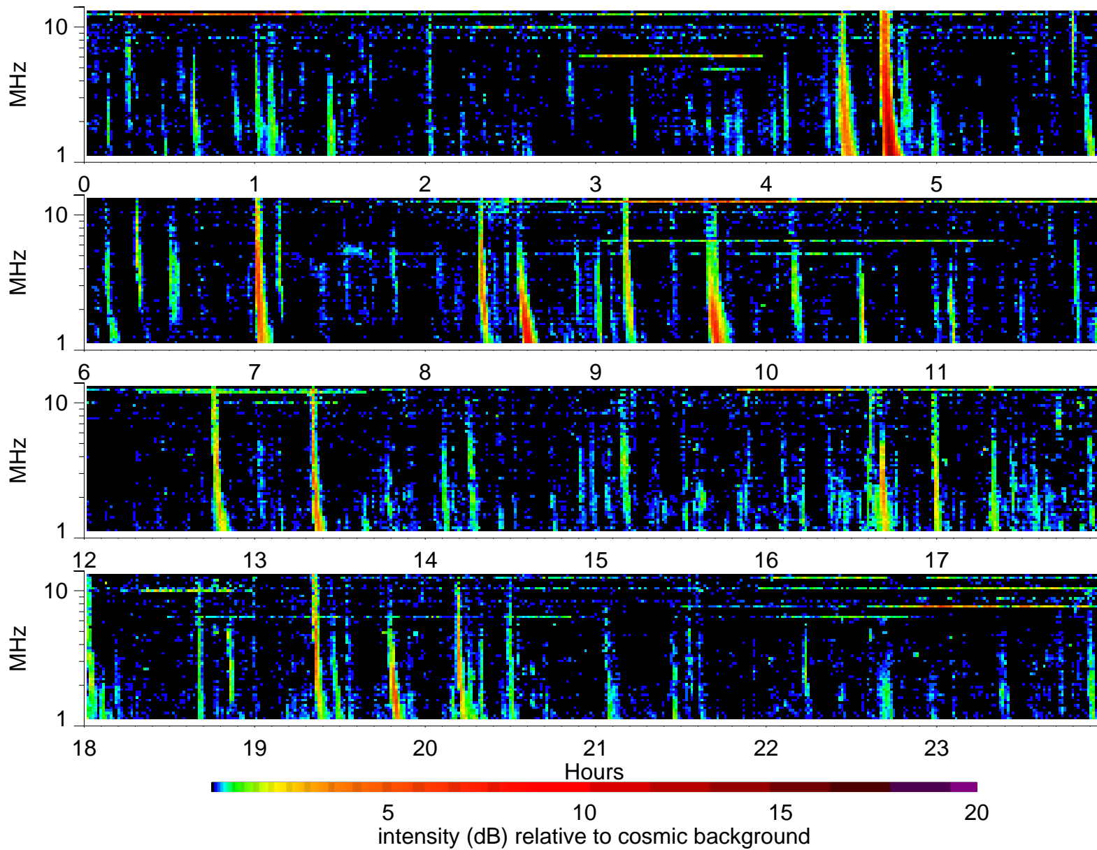
Wind Waves RAD2 receiver: 2001/4/19
