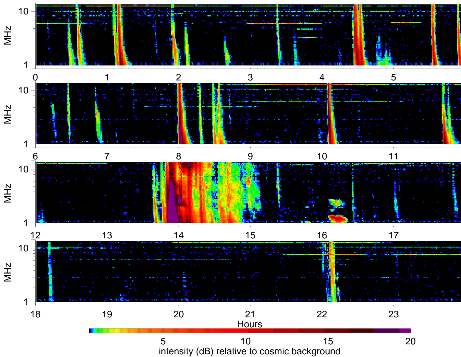
Wind Waves RAD2 receiver: 2001/4/15
