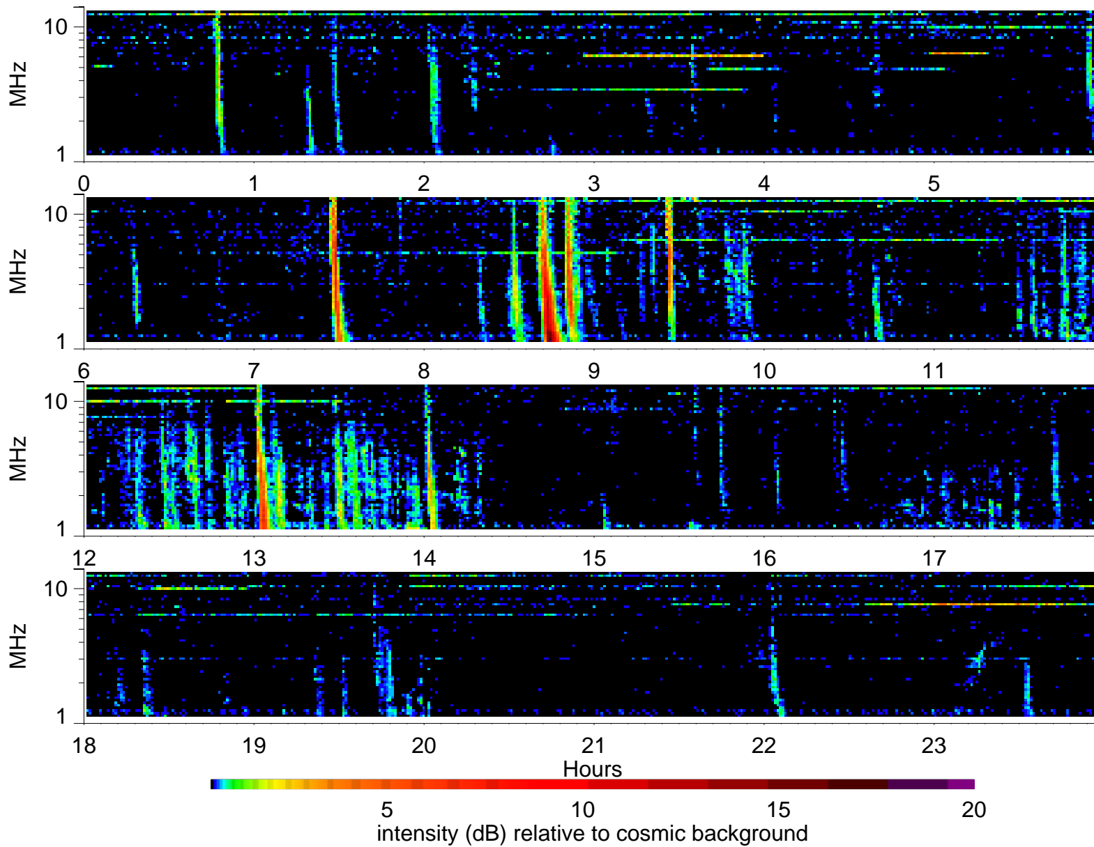
Wind Waves RAD2 receiver: 2001/4/13
