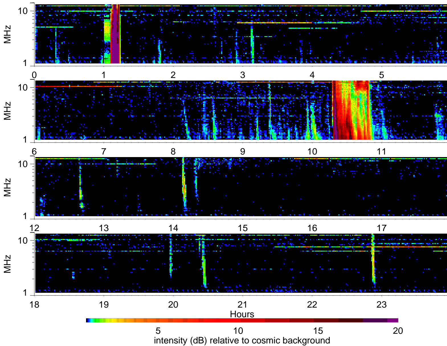
Wind Waves RAD2 receiver: 2001/4/12
