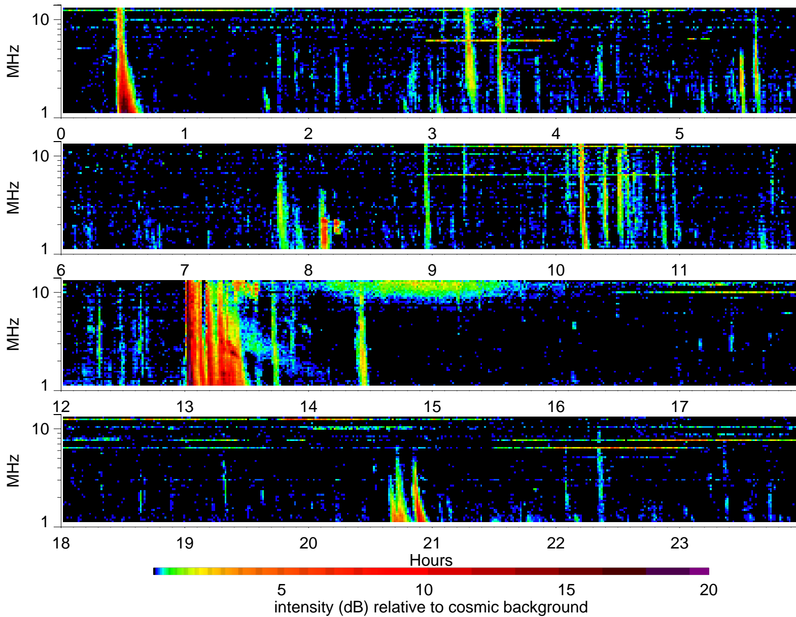
Wind Waves RAD2 receiver: 2001/4/11
